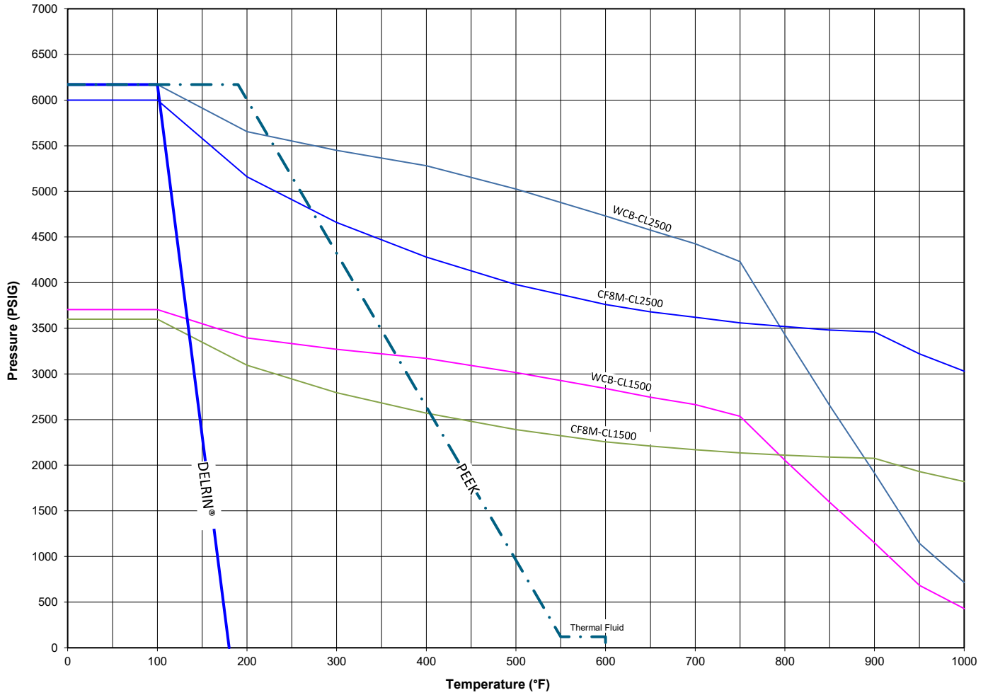
Pressure-Temperature Ratings Series 60
