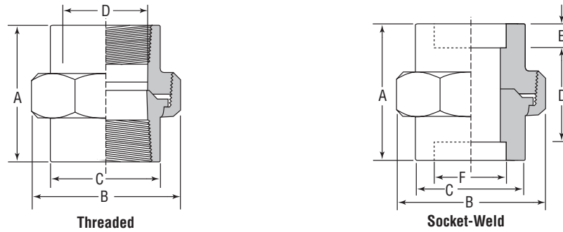
FIGURE 2127: Threaded Union
